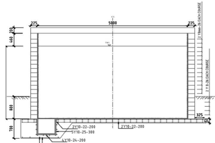
SECTION THRO' CENTRE OF TANK SCALE 1:50
